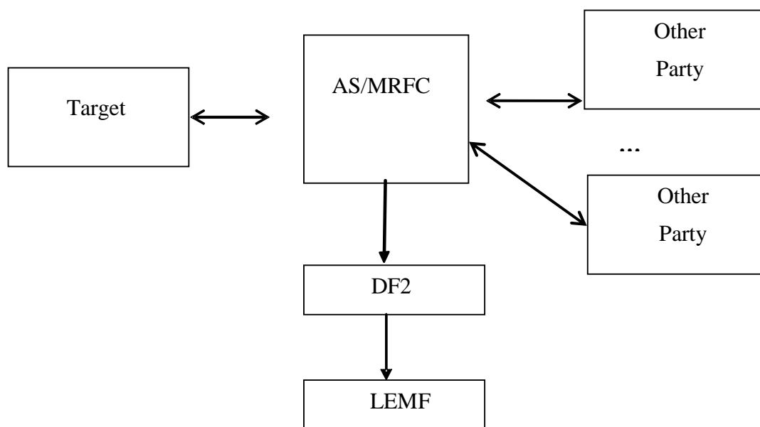
Figure 11.2: Provision of Intercept Related Information for IMS Conferencing
