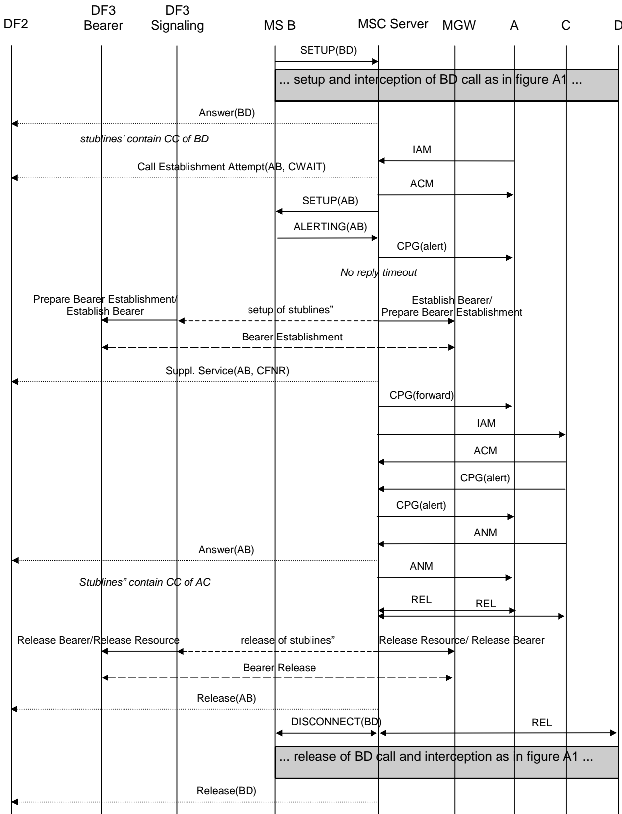
Figure A.10: Interception of call waiting / call forwarding on no reply - stblines per target
