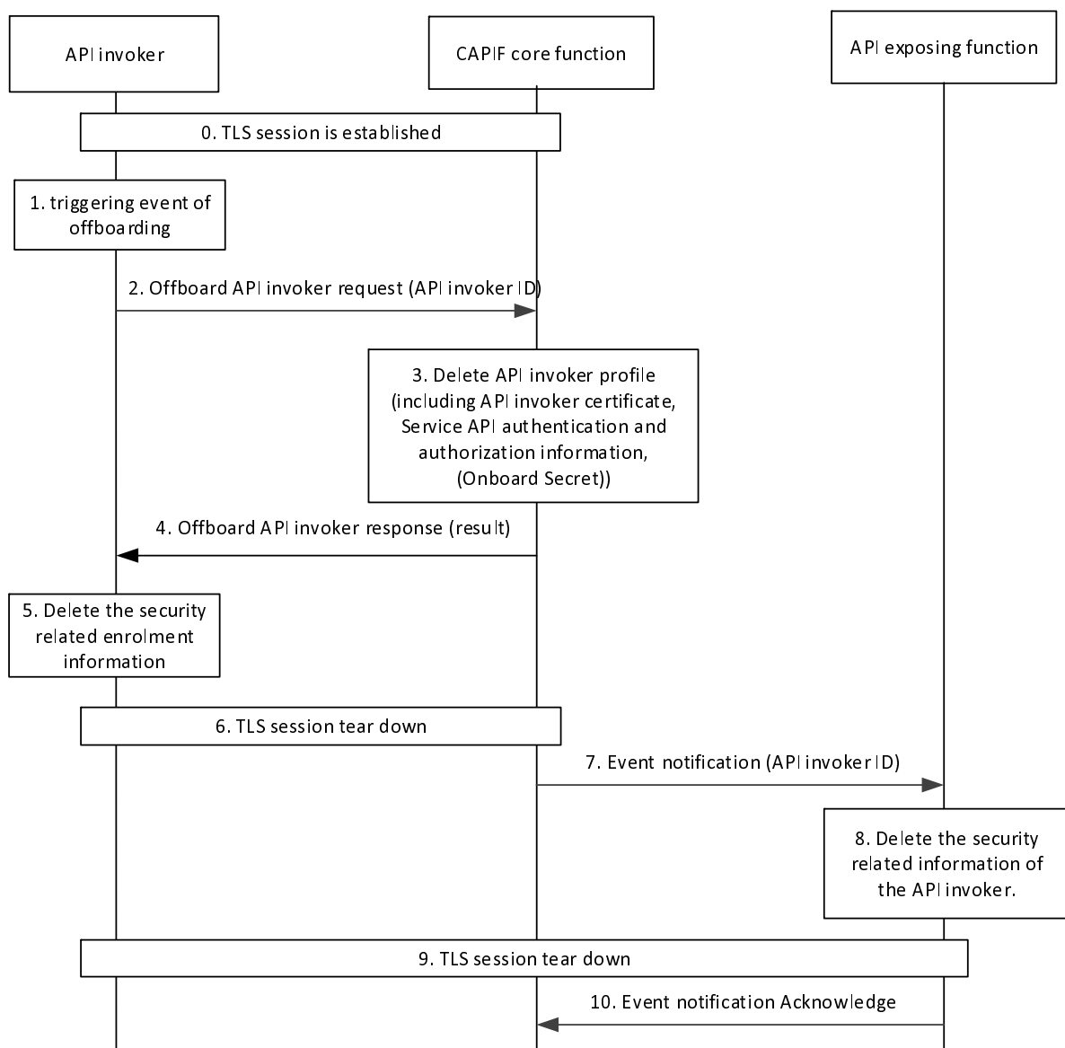
Figure 6.8-1: Security procedure for API invoker offboarding
