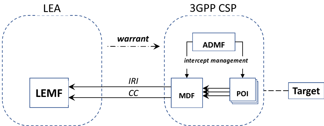
Figure 5.2: Generic Lawful Interception model
