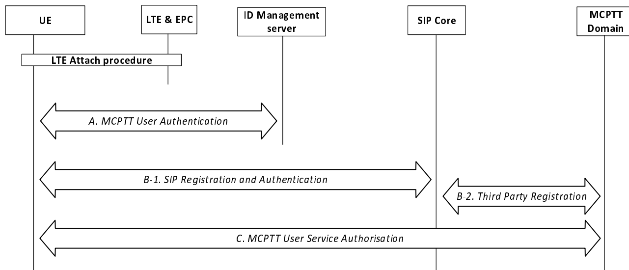
Figure 5.1-1: MCPTT Authentication
