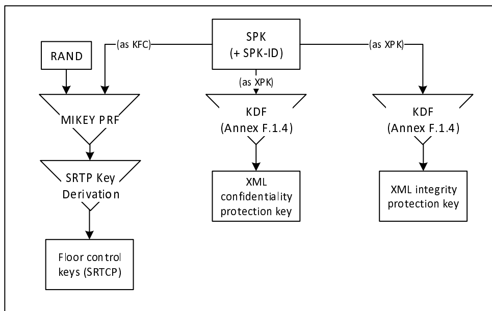
Figure 9.2-1: Uses of the Signalling Protection Key
