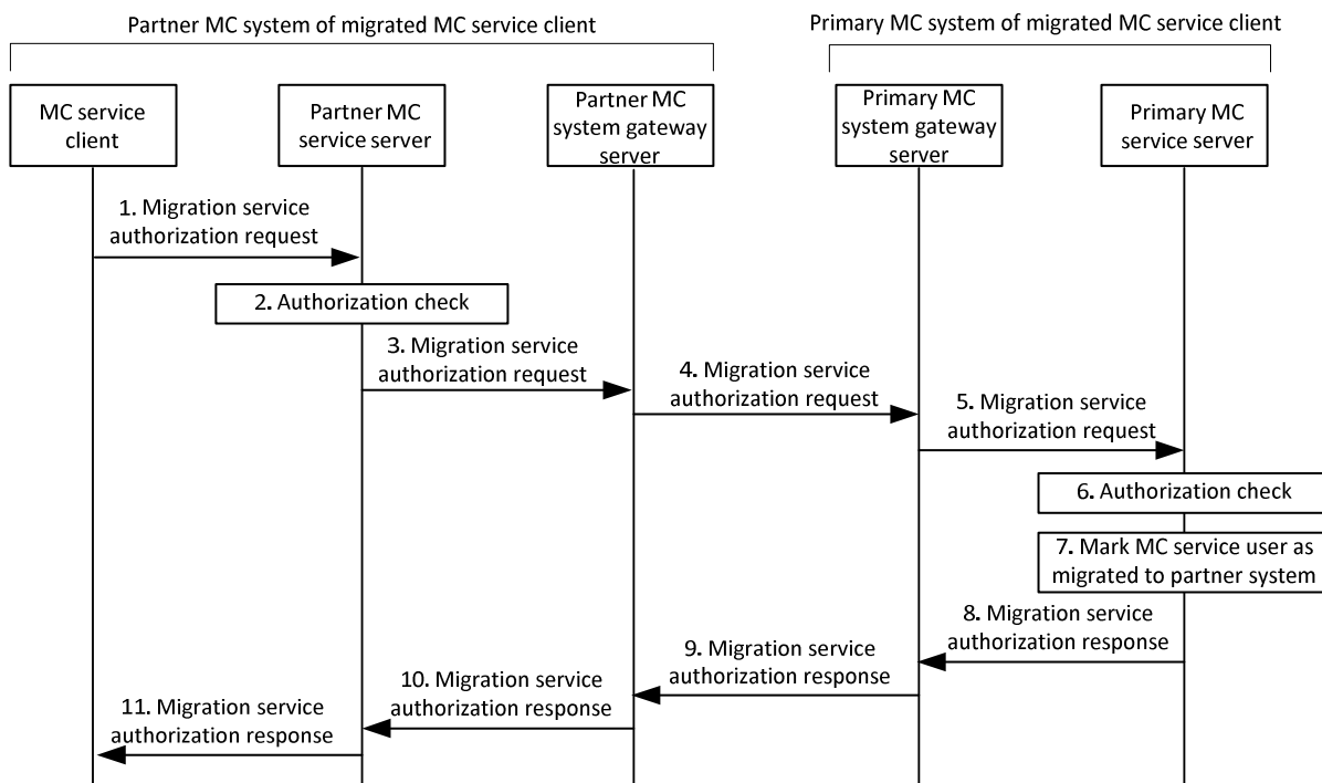
Figure 5.1.5-2 Service authorization for migration to partner MC system
