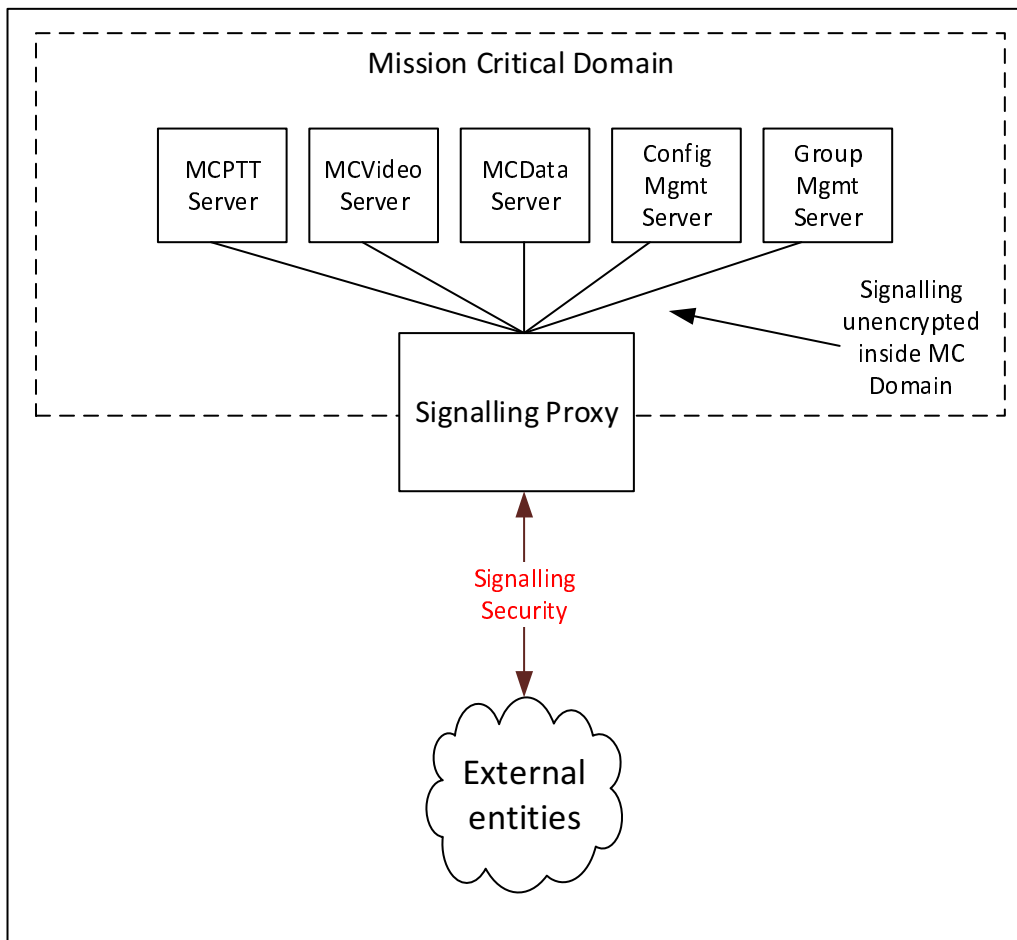
Figure 4.3.4.2-1: Signalling Proxies
