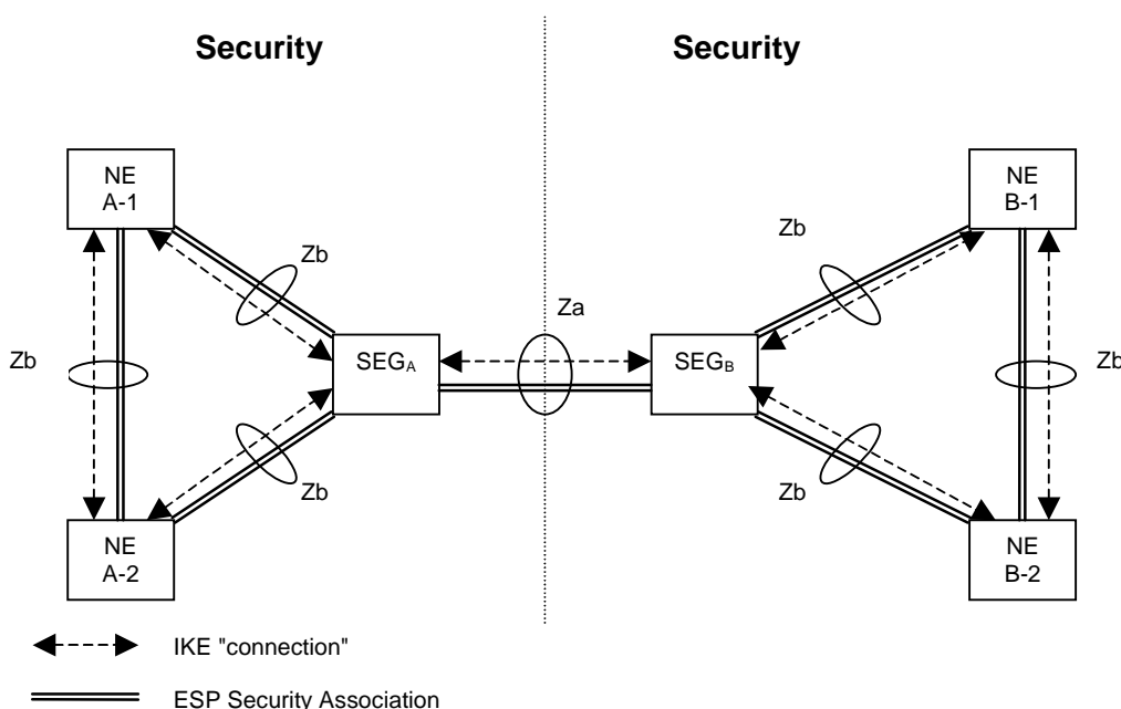
Figure 1: NDS architecture for IP-based protocols
