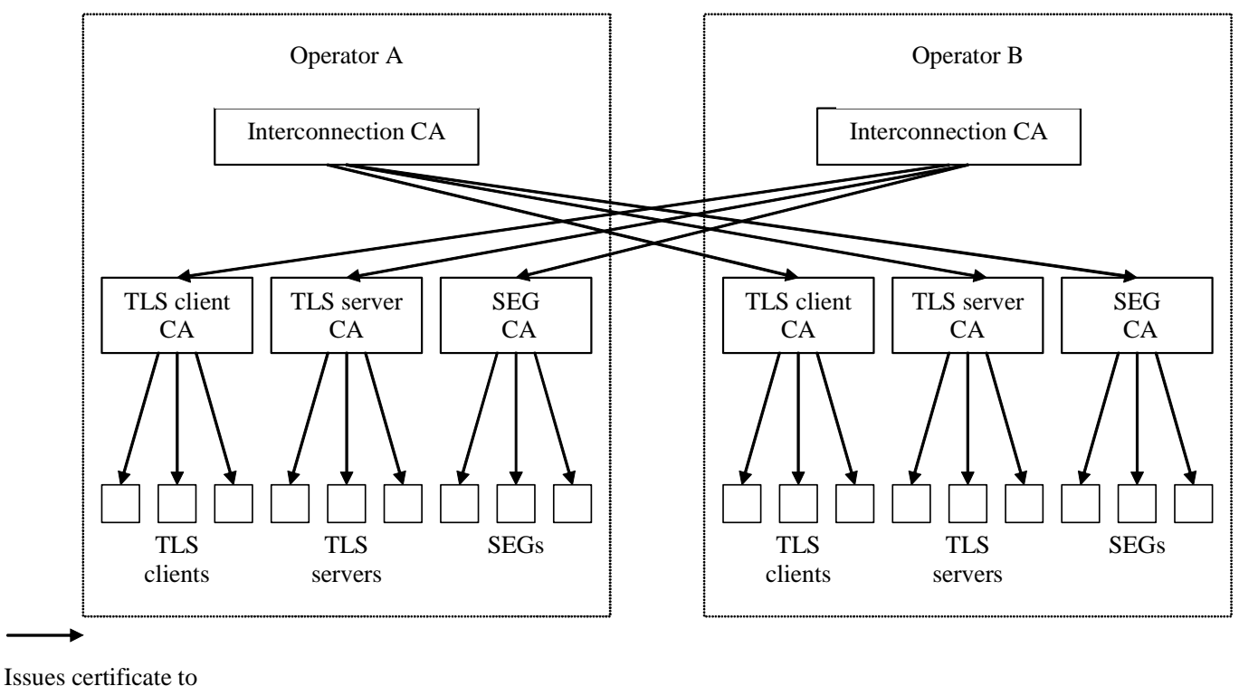
Figure 3: Certificate Hierarchy
