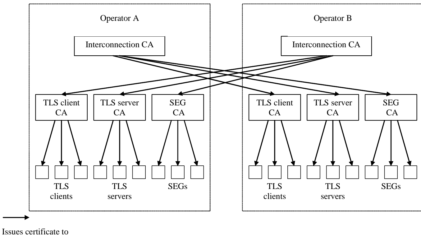
Figure 3: Certificate Hierarchy
