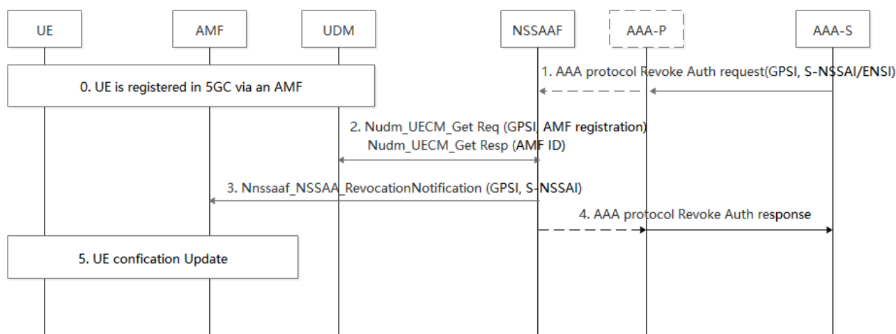
Figure 16.5-1: AAA Server-initiated Network Slice-Specific Authorization Revocation procedure
