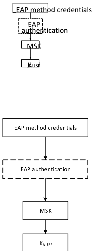
Figure I.2.3.2-1: K_{AUSF} derivation for primary authentication towards an external Credentials holder using AAA server
