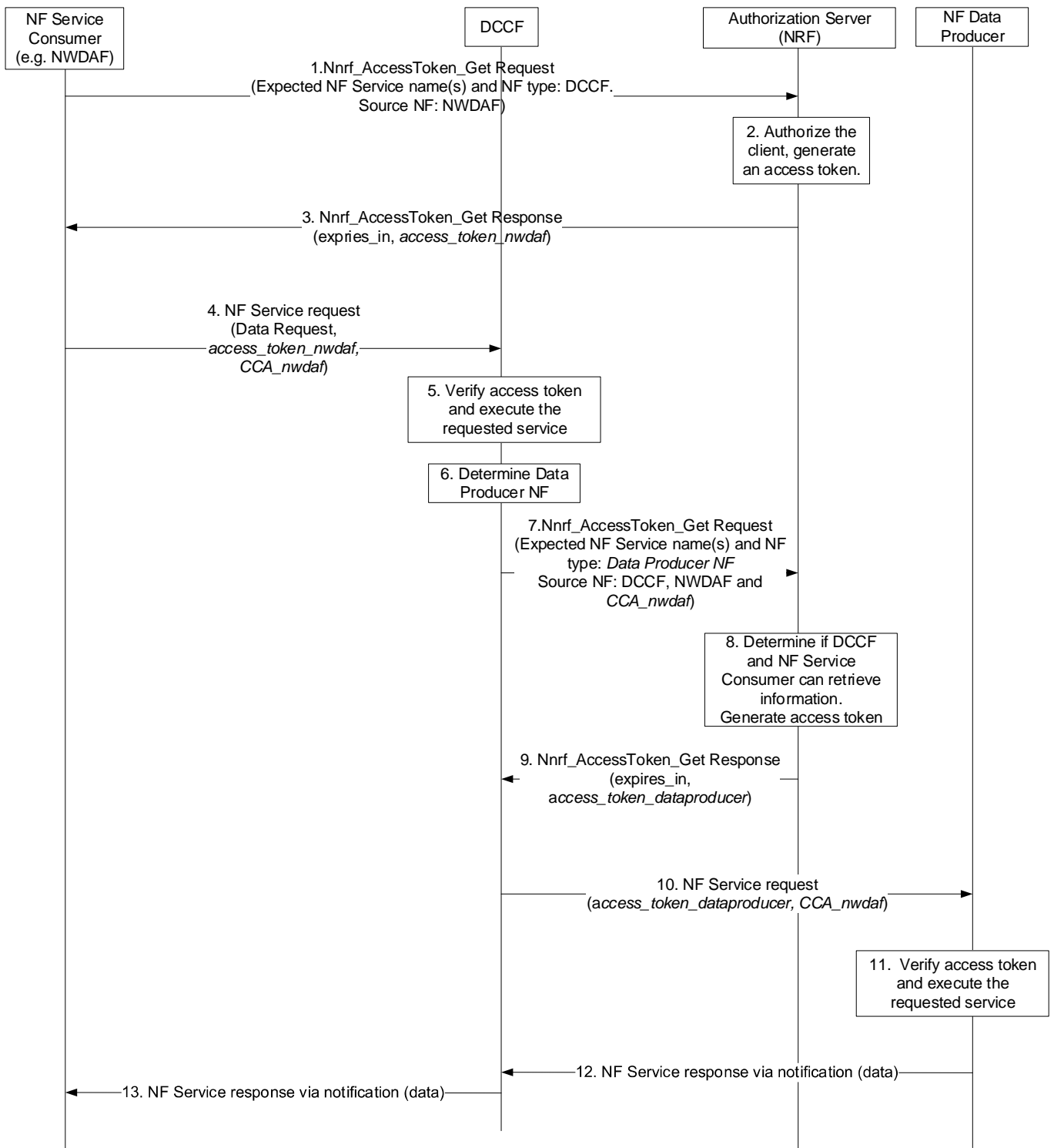
Figure X.2-1: Service Consumer Authorization to receive data from Service Producers via DCCF
