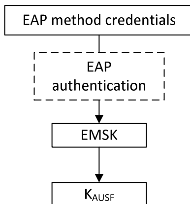
Figure I.2.3.1-1: K_{\text{AUSF}} derivation for key-generating EAP authentication methods other than EAP-AKA'
