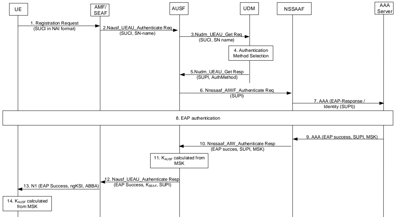
Figure: 1.2.2.2.2-1: Primary authentication with external domain
