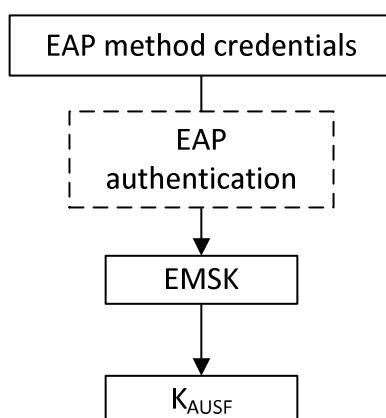
Figure I.2.3.1-1: K_{\text{AUSF}} derivation for key-generating EAP authentication methods other than EAP-AKA'
