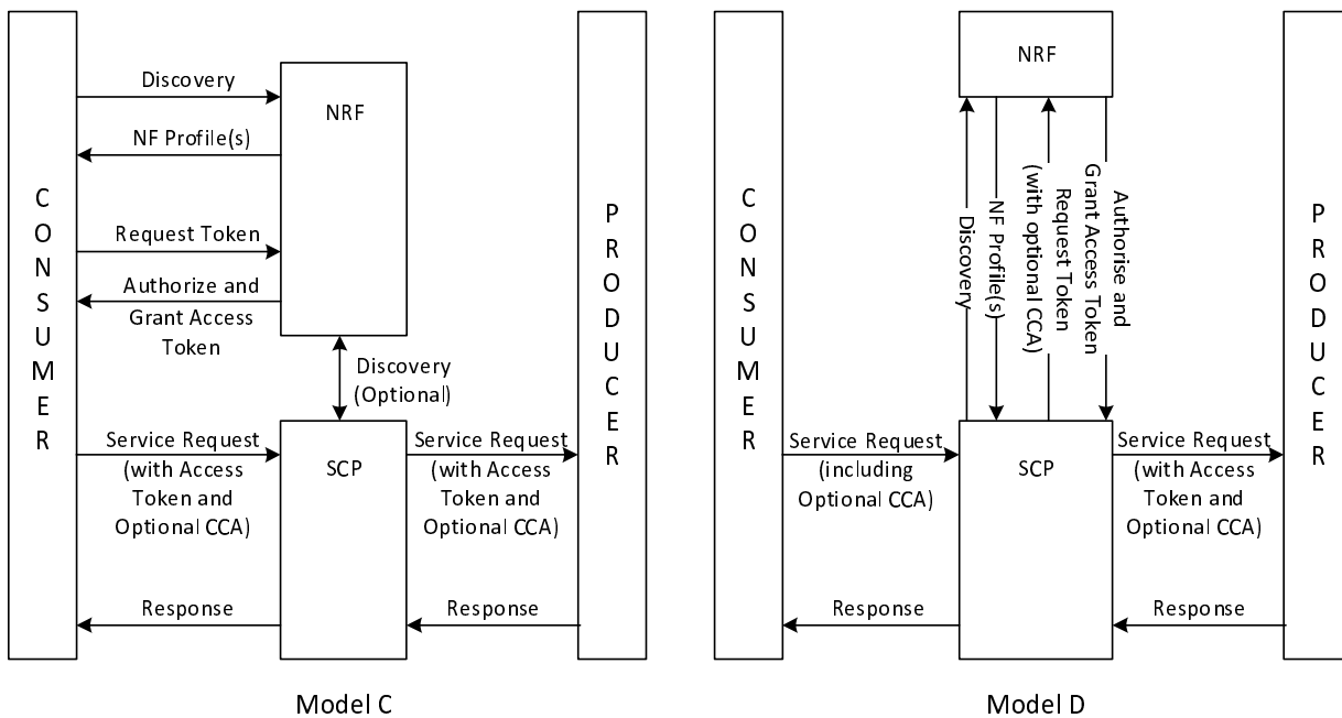
Figure R-2: Illustration of authorization aspects in indirect deployment models
