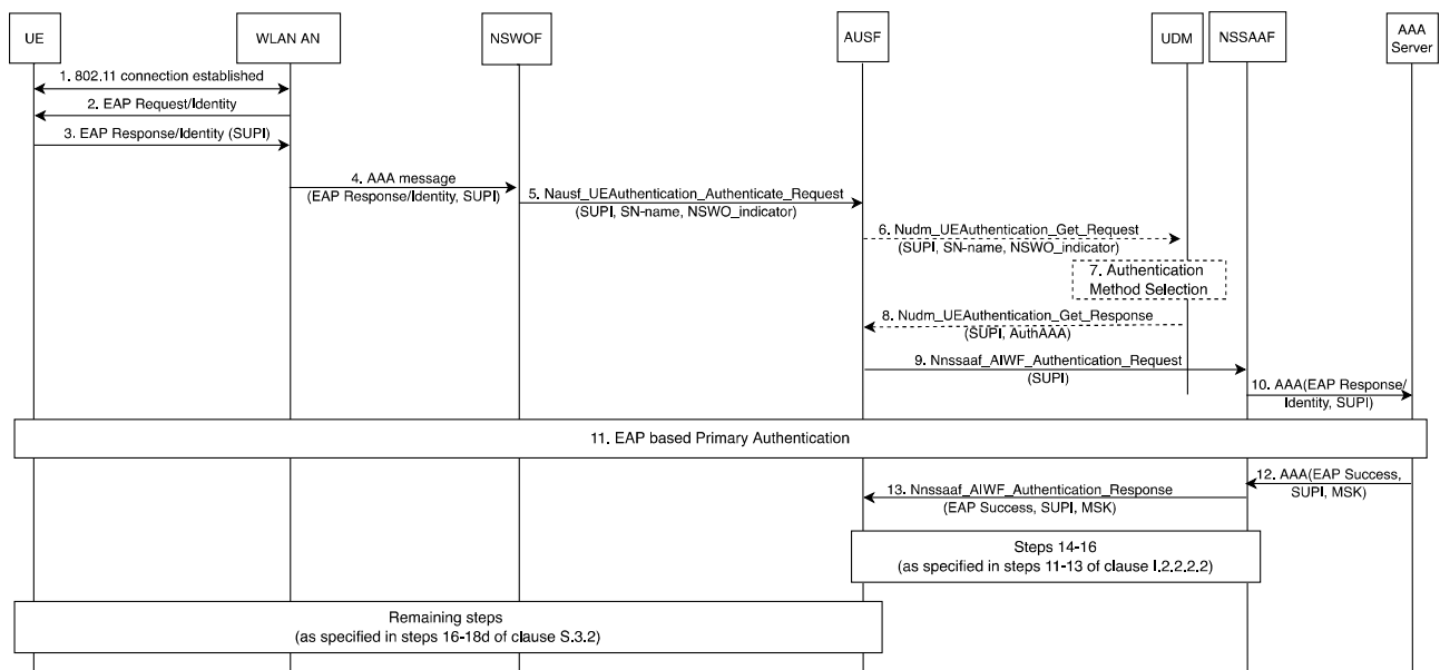
Figure I.10.5.1.2-1 - Procedure for NSWO authentication using CH with AAA server via 5GC
