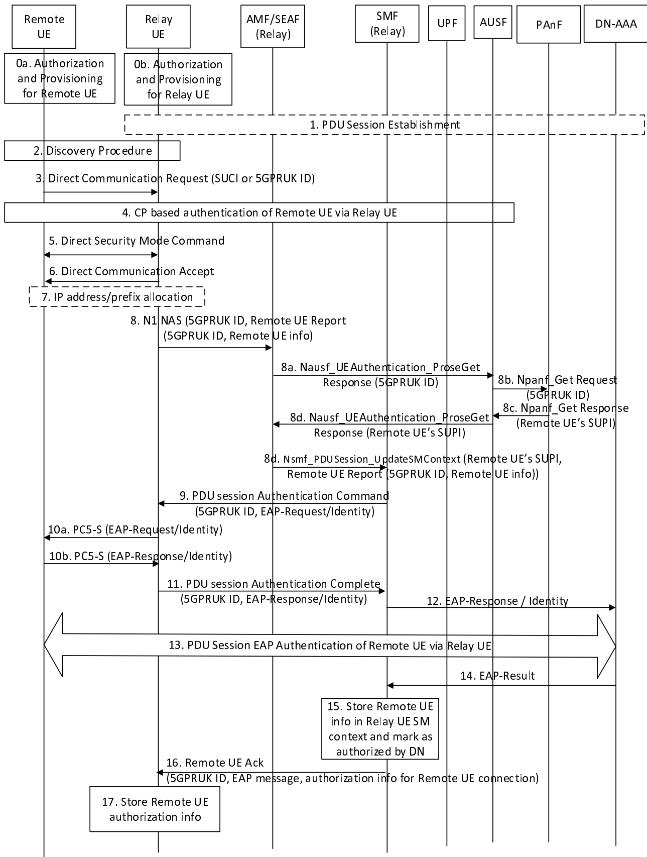
Figure 6.3.3.4.2-1: Procedure for PDU session secondary authentication of 5G ProSe Remote UE via 5G ProSe Layer-3 UE-to-Network Relay
