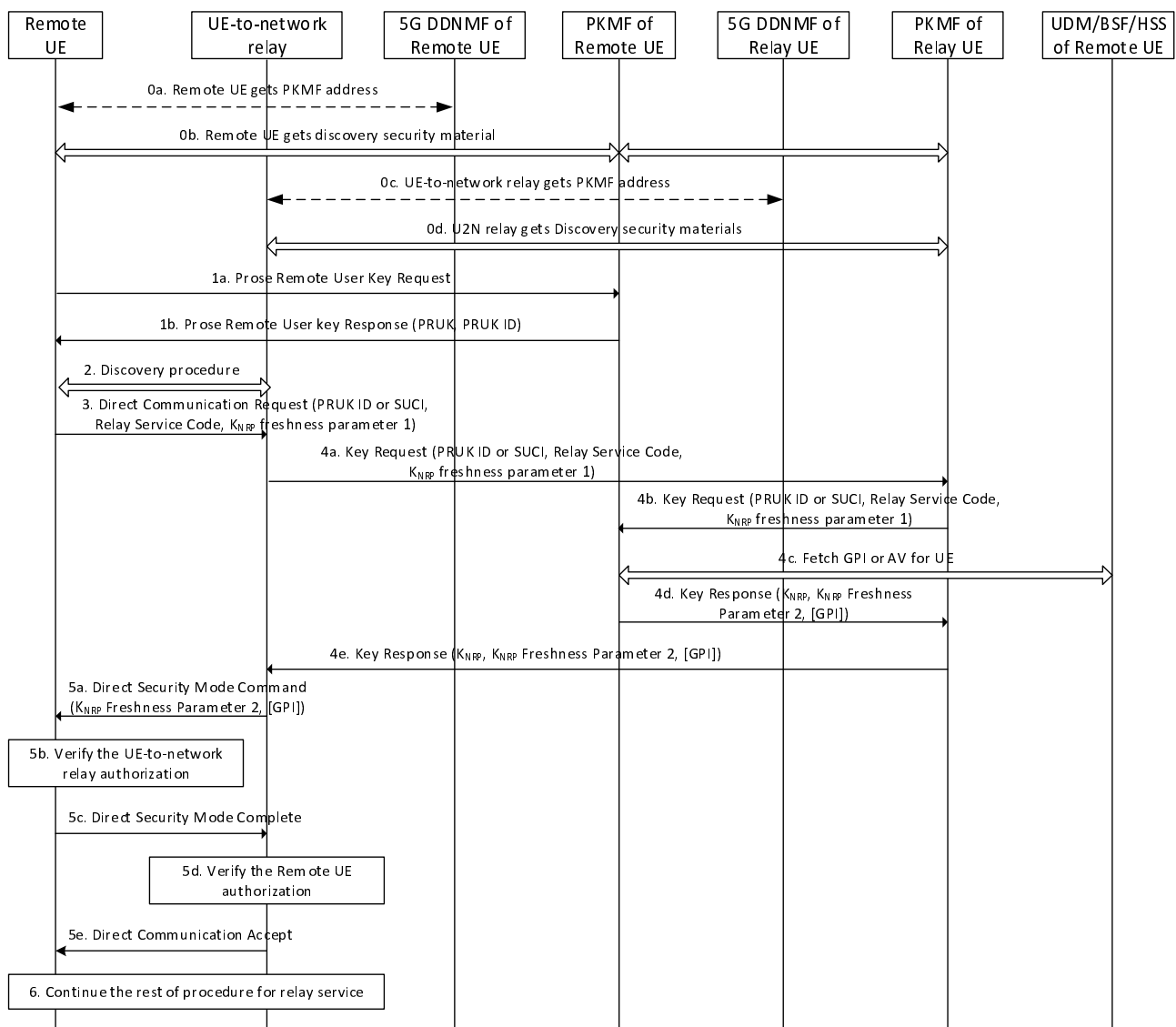
Figure 6.3.3.2.2-1: Authorization and secure PC5 link establishment procedure for 5G ProSe UE-to-Network Relay
