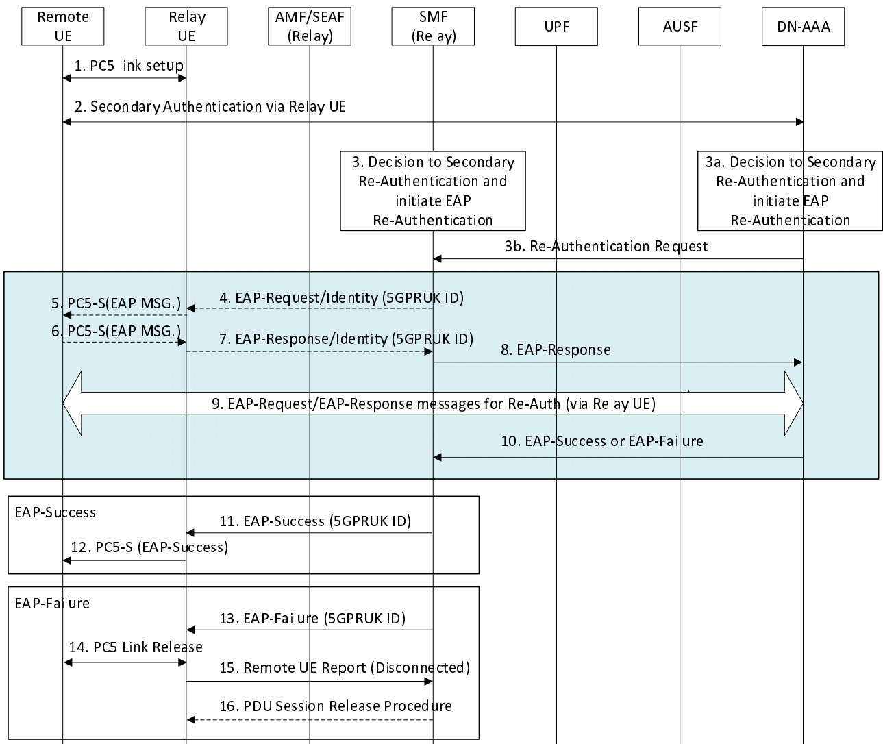
Figure 6.3.3.3.4.3-1: EAP Re-Authentication of Remote UE via L3 UE-to-Network Relay with an external AAA server
