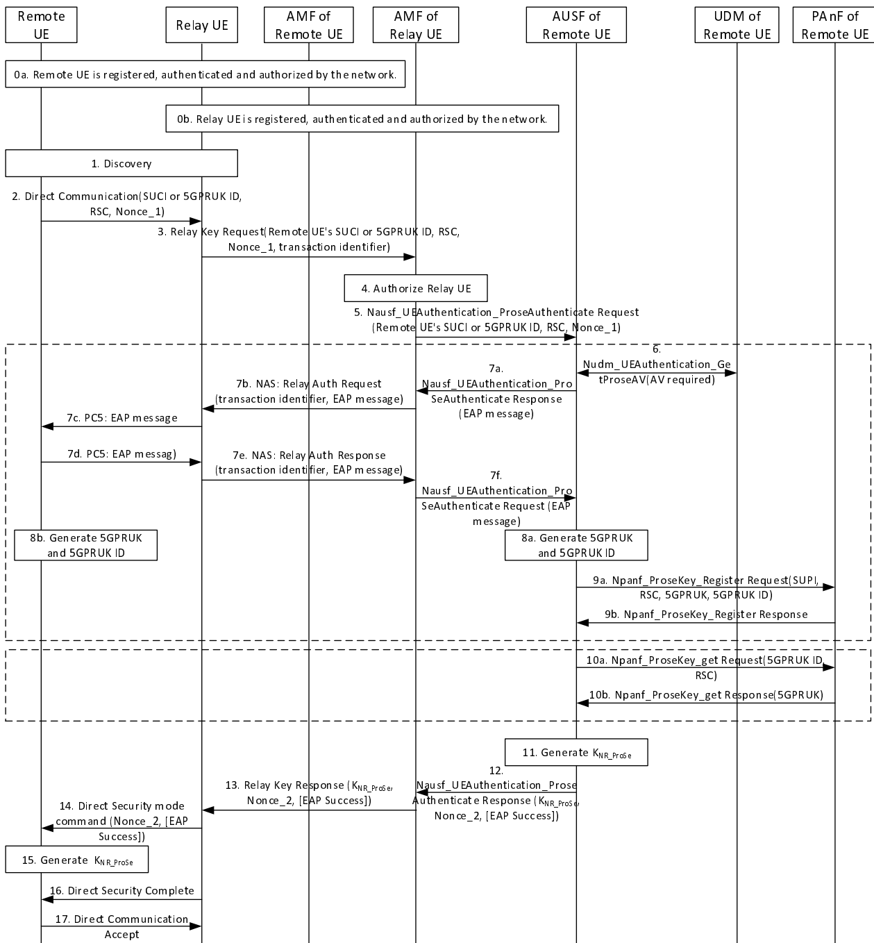
Figure 6.3.3.2-1: 5G ProSe UE-to-Network Relay security procedure with setup of network Prose security context during PC5 link establishment
