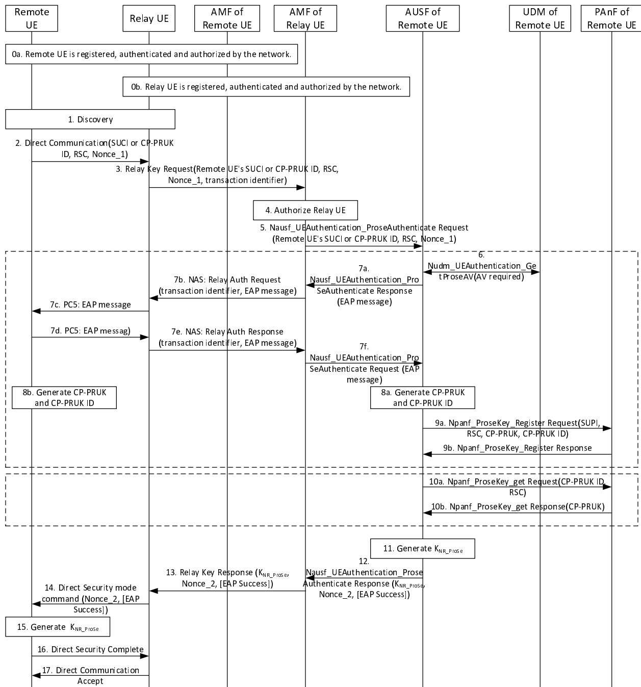
Figure 6.3.3.3.2-1: PC5 security establishment procedure for 5G ProSe UE-to-Network relay communication over Control Plane
