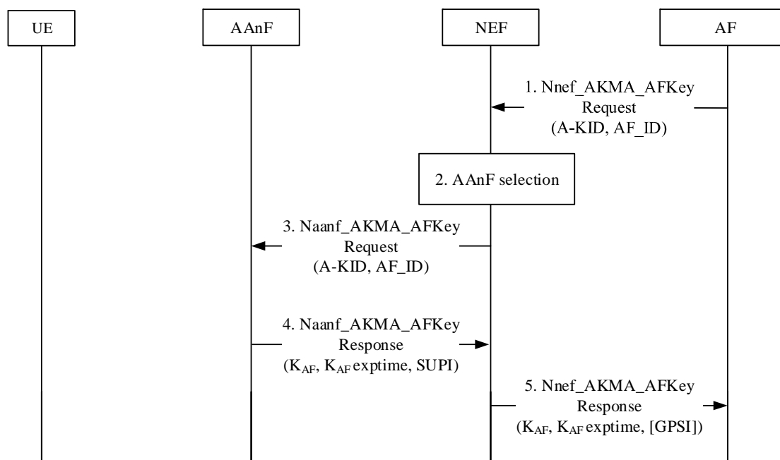
Figure 6.3-1: AKMA Application Key request via NEF
