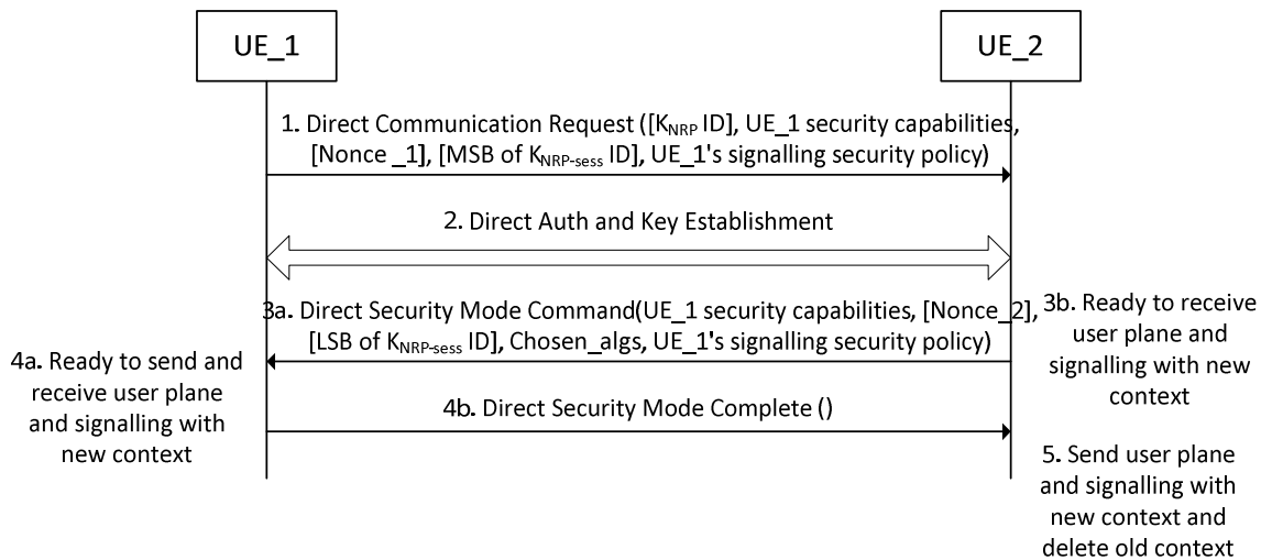
Figure 5.3.3.1.4.3-1: Security establishment at connection set-up
