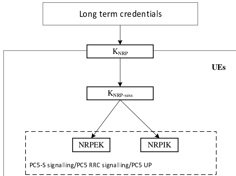
Figure 5.3.3.1.2.1-1: Key Hierarchy for PC5 unicast link
