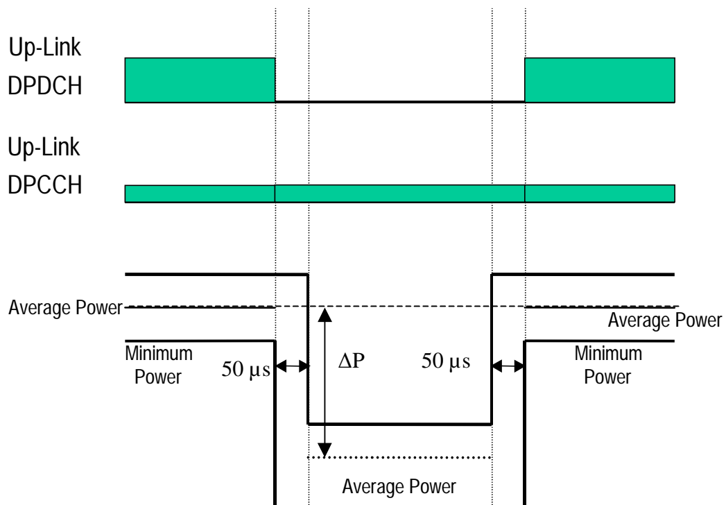
Figure 5.6.2: Transmit template during DTX
