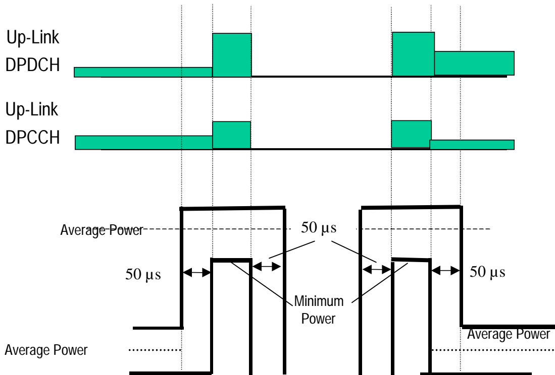
Figure 5.7.1: Transmit template during Compressed mode
