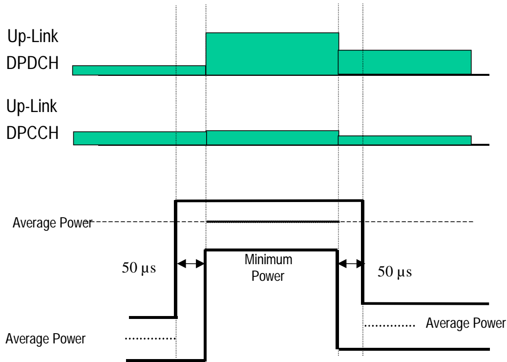
Figure 5.6.1: Transmit template during TFC change
