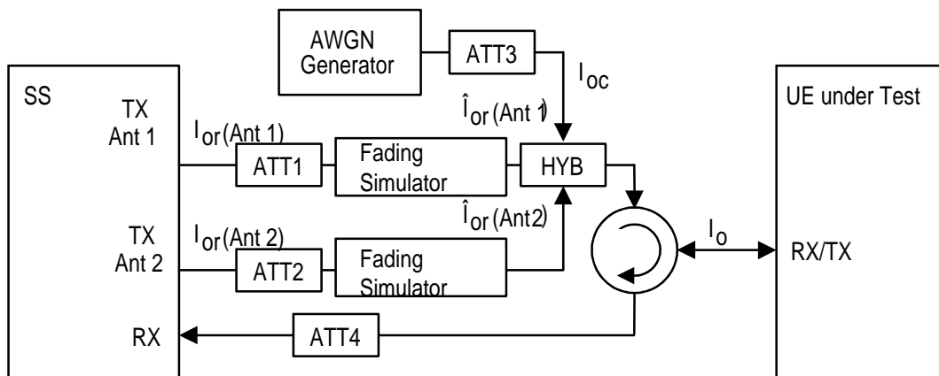
Figure A.12: Connection for Demodulation of DCH in open and closed loop transmit diversity modes
