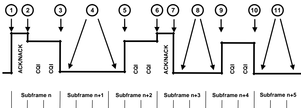
Figure 5.7A.2: Transmit power template below max power with \text{TPC\_cmd} = 0
