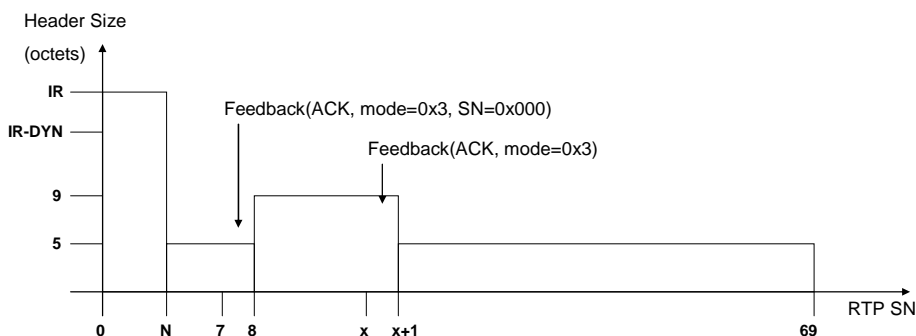
Figure 7.3.6.3: Expected outcome for ROHC RTP R-mode compressor test
