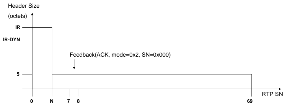
Figure 7.3.6.2: Expected outcome for ROHC RTP O-mode compressor test
