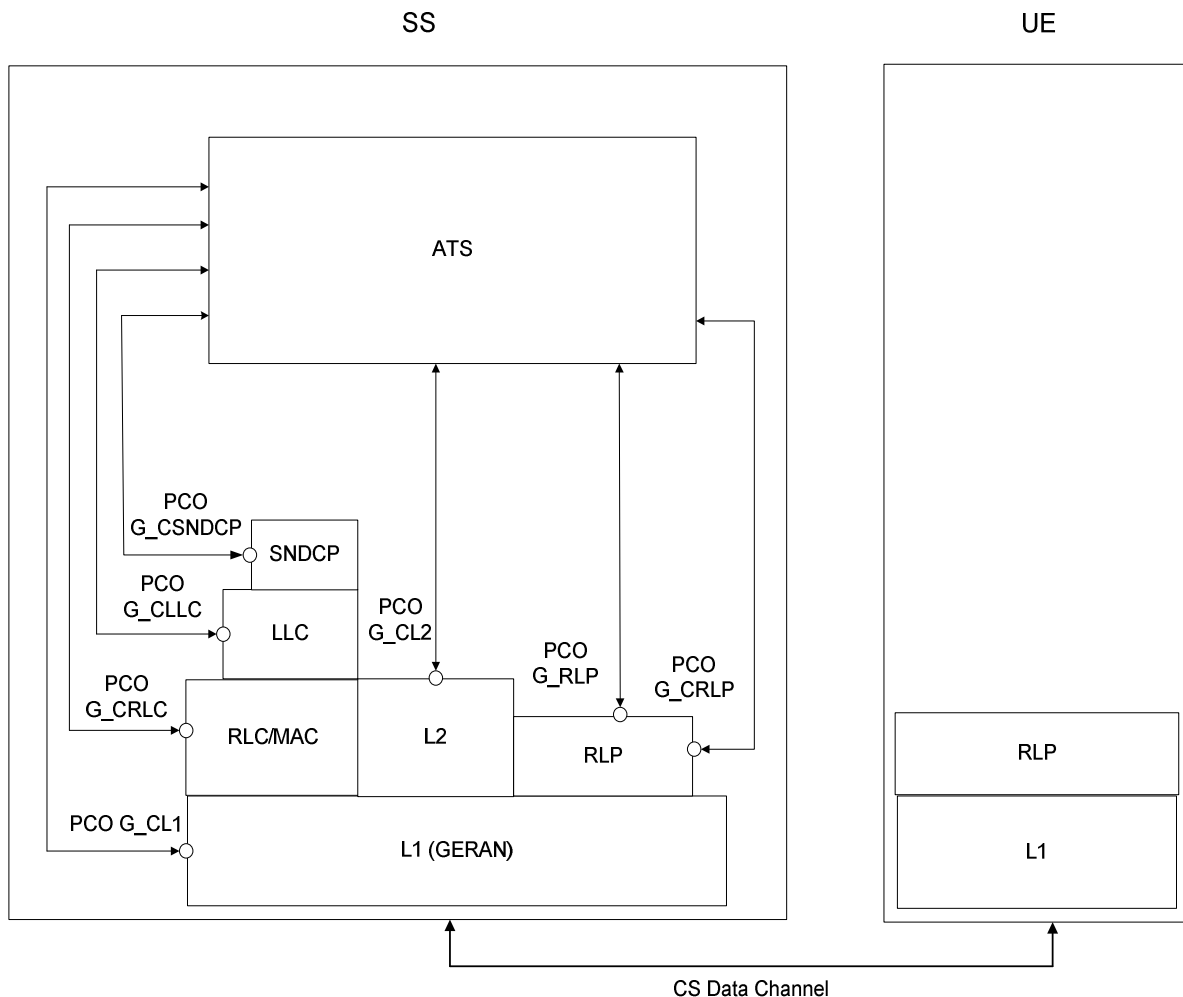
Figure 26: GERAN RLP codec model
