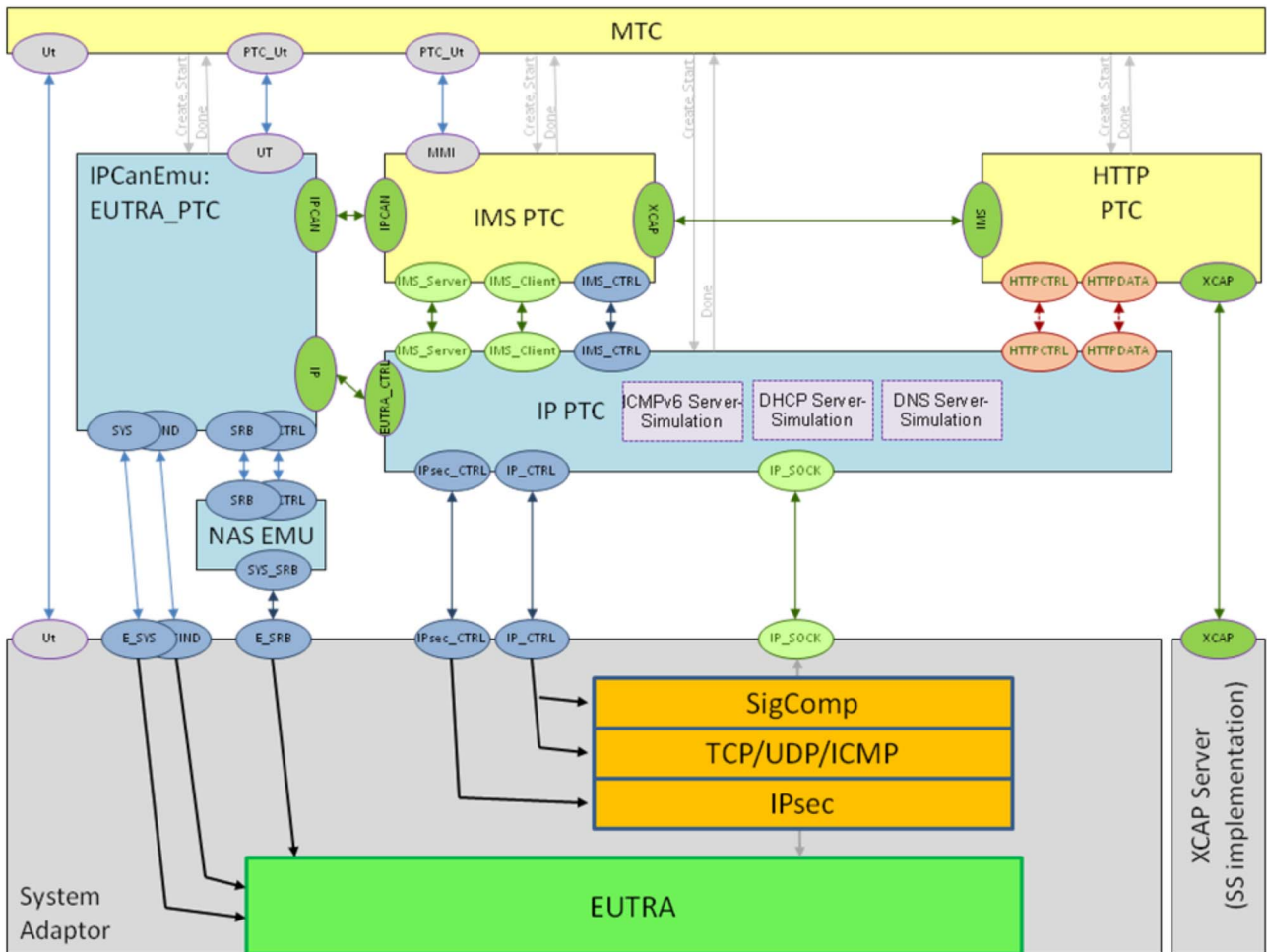
Figure 5.2-1a: Multi-TestersTest Model to support E-UTRA SS interface
