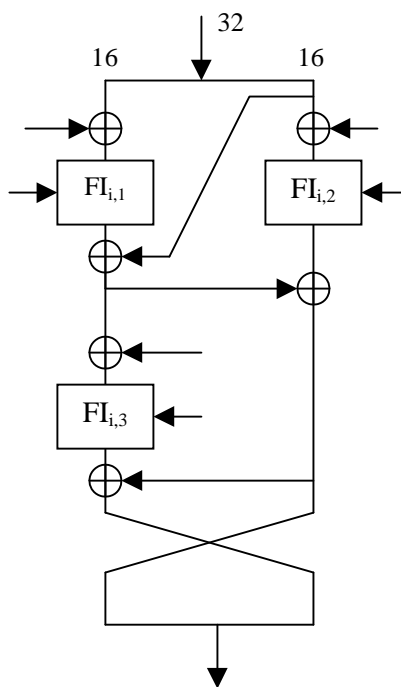
Fig.6: FO Function
