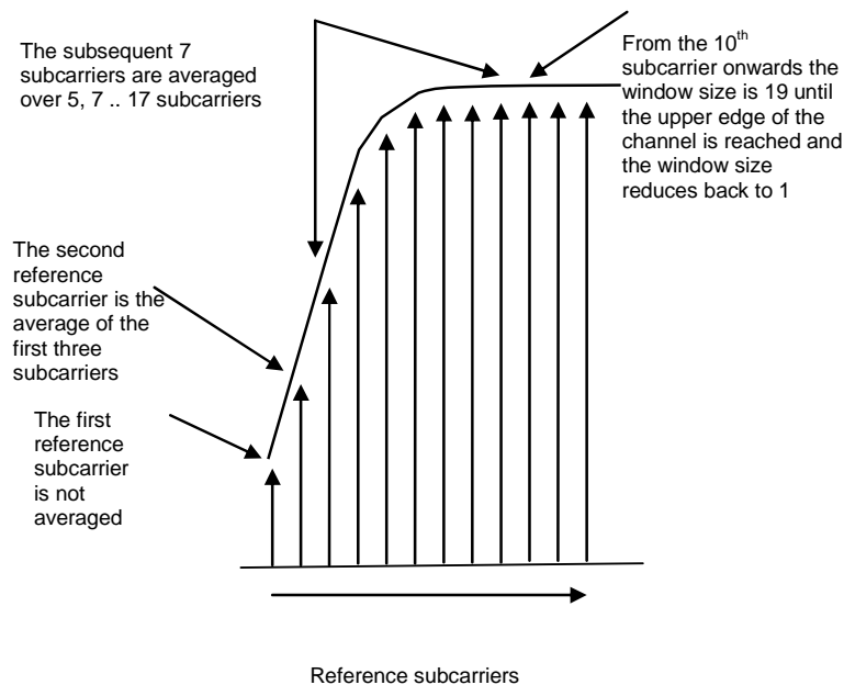
Figure E.6-1: Reference subcarrier smoothing in the frequency domain
