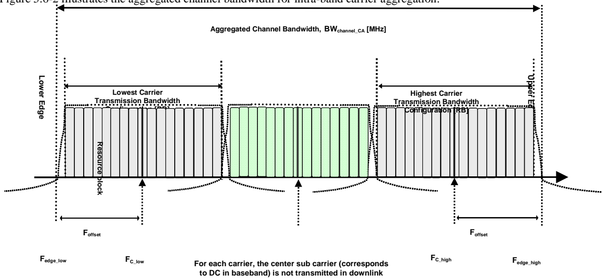
Figure 5.6-2 Definition of Aggregated Channel Bandwidth for intra-band carrier aggregation
