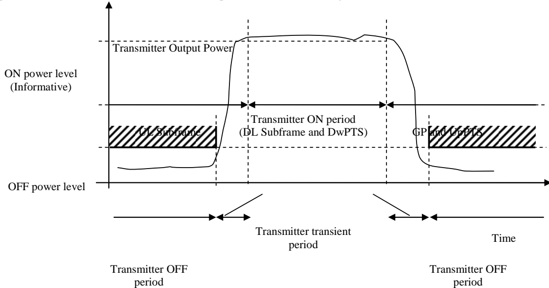
Figure 6.4.2-1 Illustration of the relations of transmitter ON period, transmitter OFF period and transmitter transient period.
