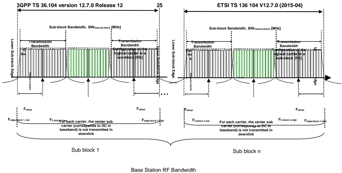
Figure 5.6-3 Definition of Sub-block Bandwidth for intra-band non-contiguous spectrum
