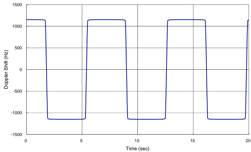
Figure B.3-2: Doppler shift trajectory for scenario 3
