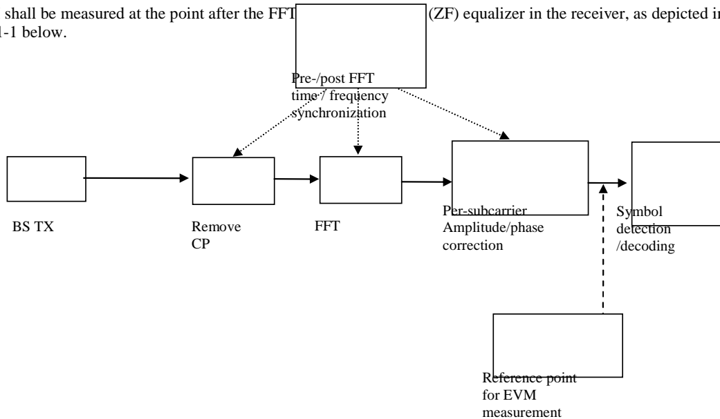
Figure E.1-1: Reference point for EVM measurement
