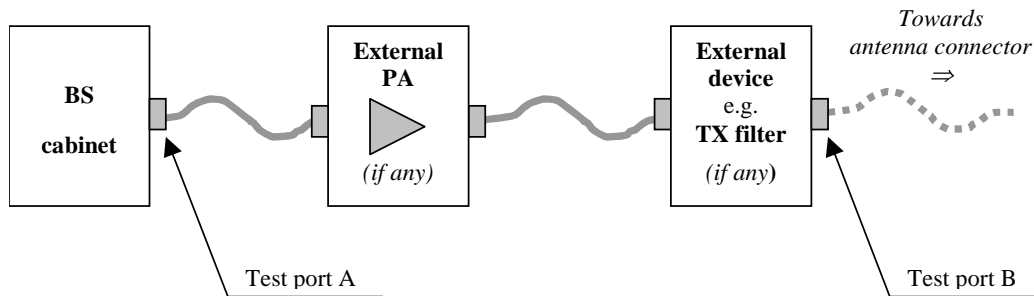
Figure 6.1-1: Transmitter test ports
