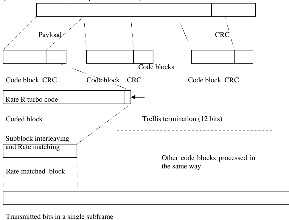
Figure A-1. Schematic overview of the encoding process
