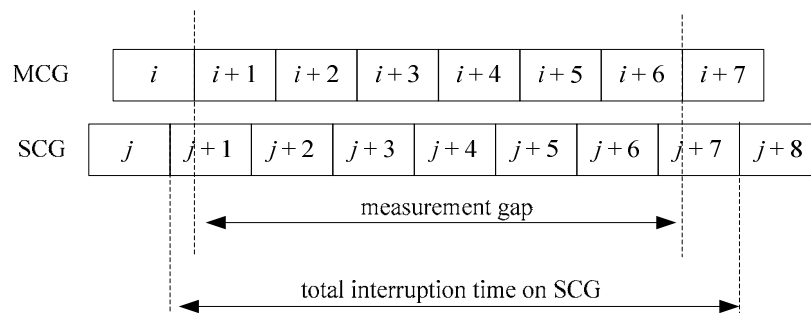
(b) measurement GAP for asynchronous dual connectivity
