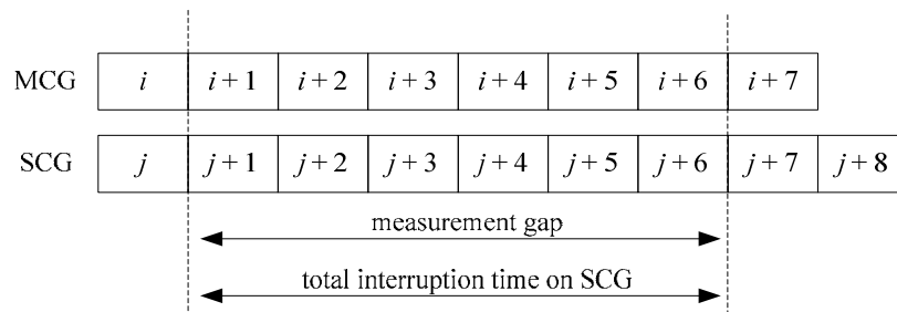
(a) measurement GAP for synchronous dual connectivity
