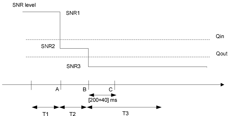
Figure A.7.3.9.1-1 SNR variation for out-of-sync testing
