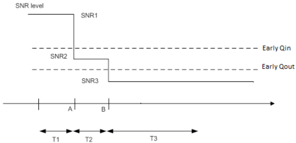
Figure A.7.3.99.1-1: SNR variation for early out-of-sync testing
