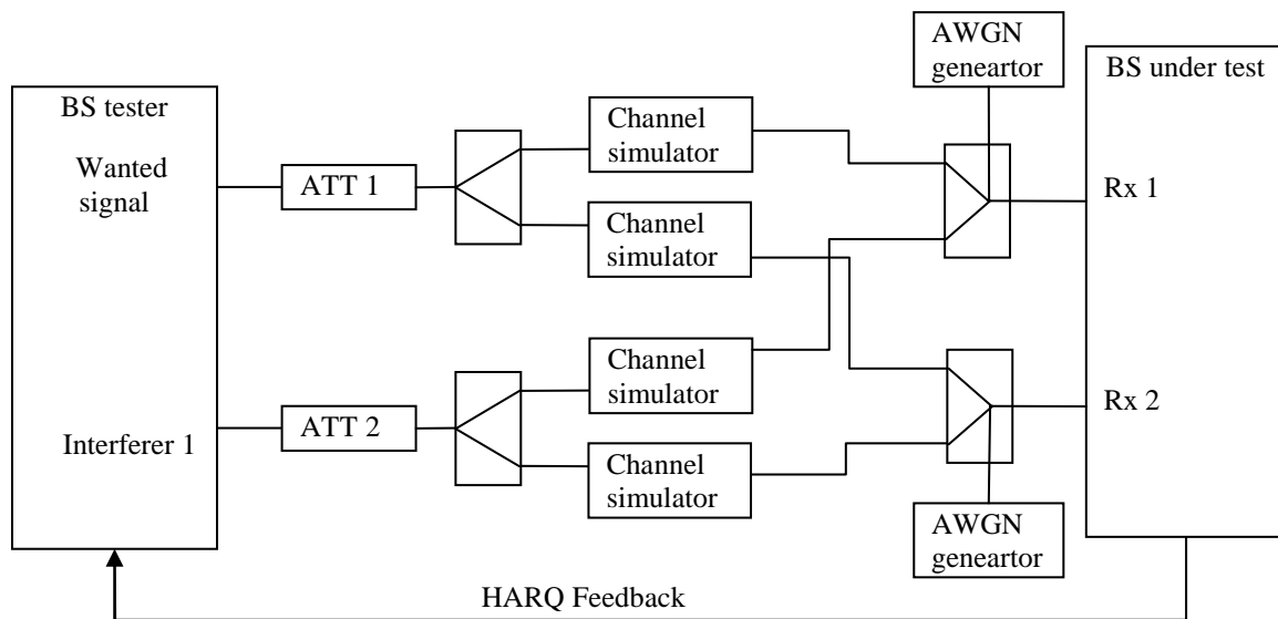
Figure I.3-7a: Functional set-up for enhanced performance requirements type A of 2Rx PUSCH in multipath fading conditions with synchronous interference (1 interferer and 2 Rx case shown)
