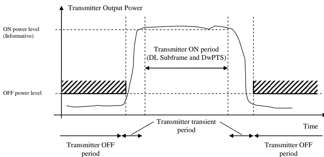
Figure 6.4.2.1-1 Illustration of the relations of transmitter ON period, transmitter OFF period and transmitter transient period.
