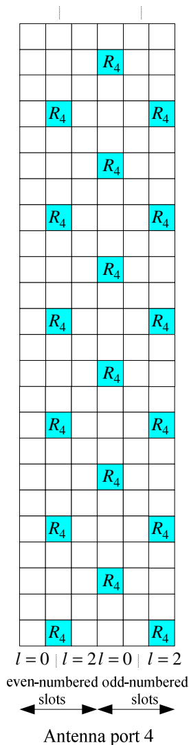
Figure 6.10.2.2-3: Mapping of MBSFN reference signals (extended cyclic prefix, \Delta f = 7.5 kHz)
