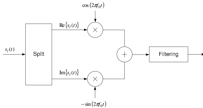
Figure 5.8-1: Uplink modulation
