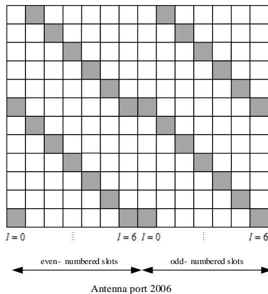
Figure 10.2.6A.2-2: Mapping of NPRS ( operationModelInfoNPRS is set to standalone or guard-band, nprsBitmap configured)
