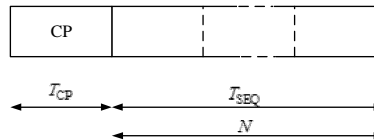
Figure 10.1.6.1-1: Random access symbol group
