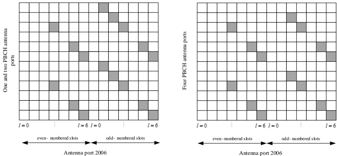
Figure 10.2.6A.2-1: Mapping of NPRS ( operationModelInfoNPRS is set to in-band, nprsBitmap configured)
