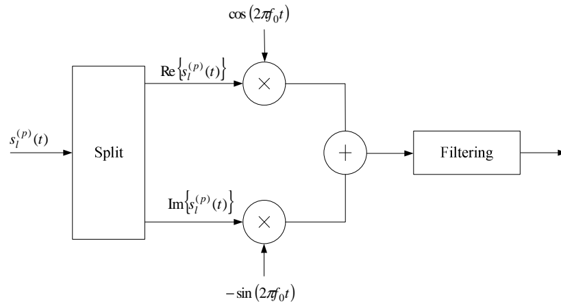
Figure 6.13-1: Downlink modulation
