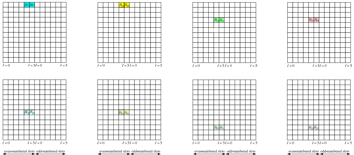
Figure 6.10.5.2-2: Mapping of CSI reference signals (CSI configuration 0, extended cyclic prefix)
