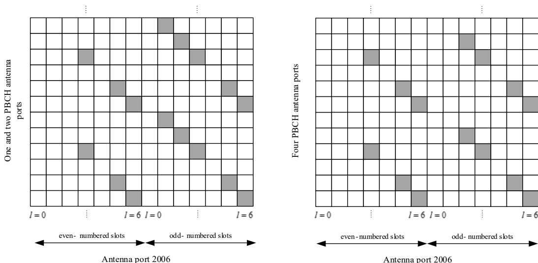
Figure 10.2.6A.2-1: Mapping of NPRS ( operationModeInfoNPRS is set to in-band, nprsBitmap configured)
