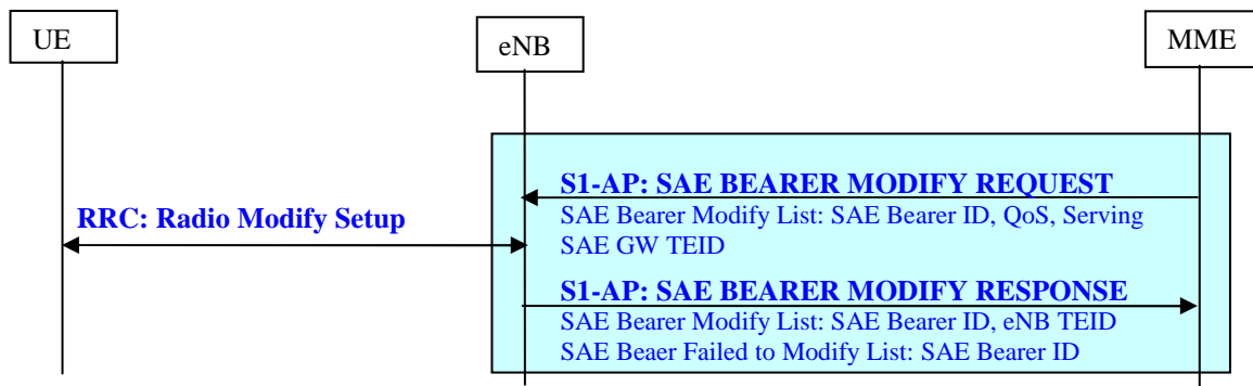
Figure 19.2.2.4.2-1: EPS Bearer Modification procedure
