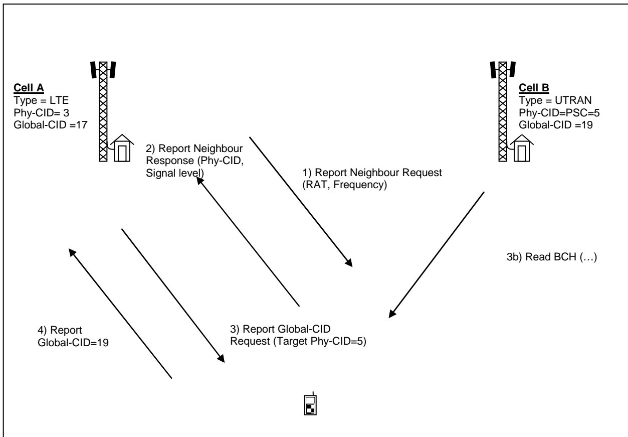
Figure 22.3.4-1: Automatic Neighbor Relation Function
