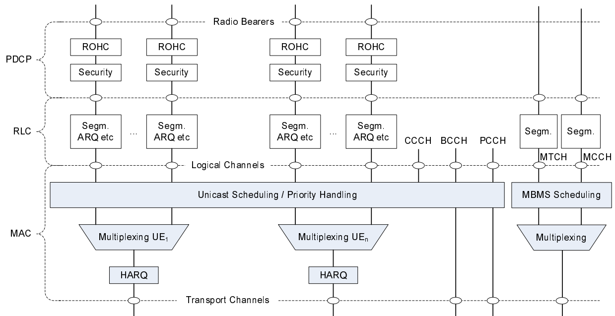
Figure 6-1: Layer 2 Structure for DL
