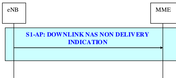
Figure 19.2.2.6-4: Downlink NAS Non Delivery Indication procedure
