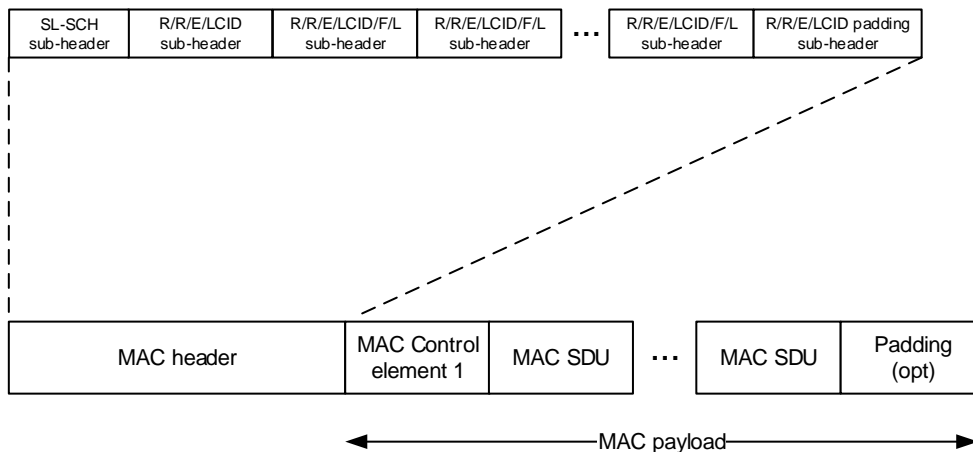
Figure 6.1.6-4: Example of MAC PDU consisting of MAC header, MAC control element, MAC SDUs and padding
