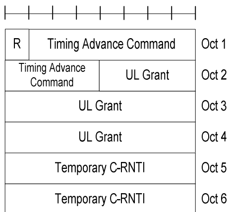
Figure 6.1.5-3: MAC RAR
