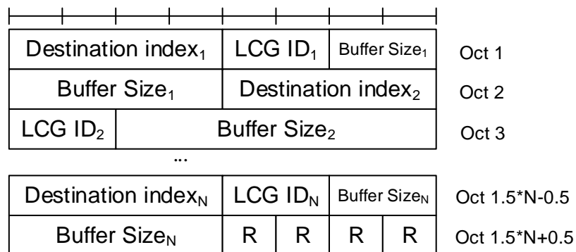
Figure 6.1.3.1a-2: Sidelink BSR and Truncated Sidelink BSR MAC control element for odd N
