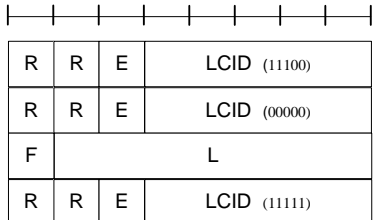
Case 5: MAC subheader for MAC control element + MAC subheader (7-bits L-field) for MAC SDU (CCCH) + MAC subheader for padding
