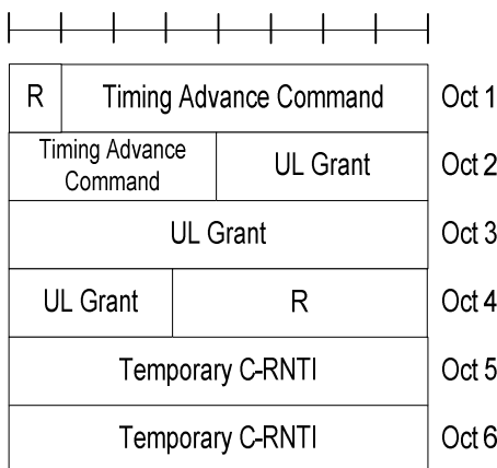
Figure 6.1.5-3b: MAC RAR for NB-IoT UEs
