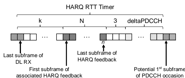
Figure C-1: Setting the HARQ RTT Timer for NB-IoT
