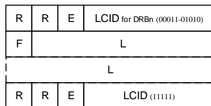
Case 8: MAC subheader for MAC control element + MAC subheader (7-bits L-field) for MAC SDU (DCCH) + MAC subheader (7or15-bits L-field) for MAC SDUs (DTCHs) + MAC subheader for padding
