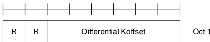
Figure 6.1.3.21-1: Differential Koffset MAC CE
