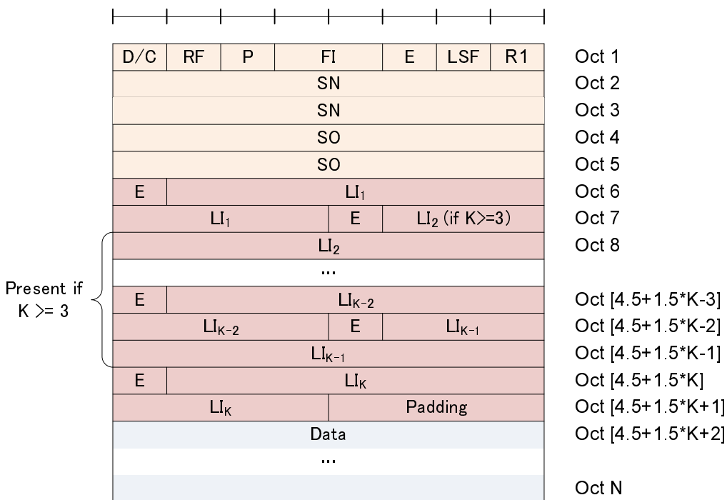
Figure 6.2.1.5-2a: AMD PDU segment with 16 bit SN and with 16 bit SO (length of LI field is 11 bits) (Odd number of LIs, i.e. K = 1, 3, 5, ...)
