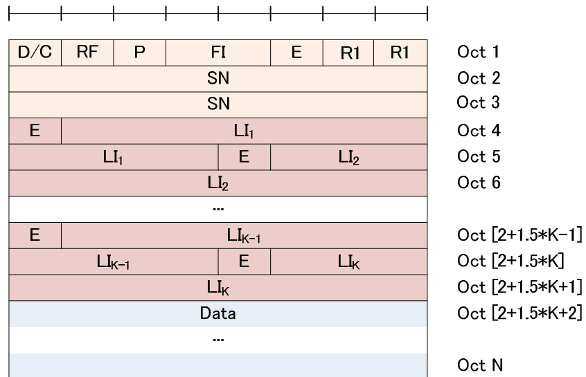
Figure 6.2.1.4-3a: AMD PDU with 16 bit SN (length of LI field is 11 bits) (Even number of LIs, i.e. K = 2, 4, 6, \dots )
