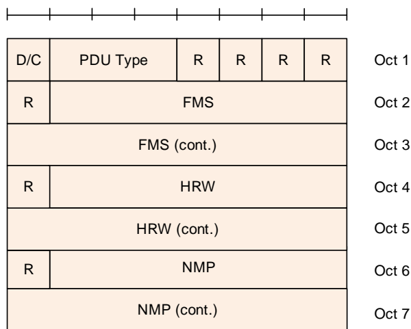
Figure 6.2.12.2: PDCP Control PDU format for LWA status report using a 15 bit SN
