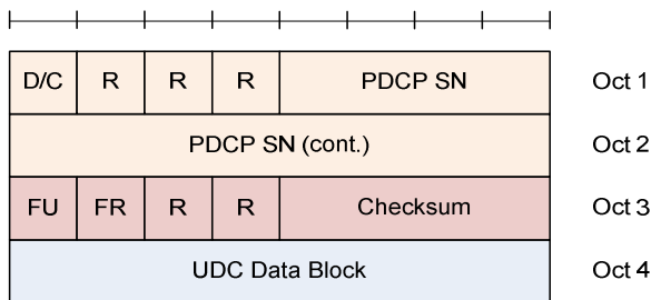
Figure 6.2.14.1: PDCP Data PDU format for DRBs using a 12 bit SN (UDC configured)
