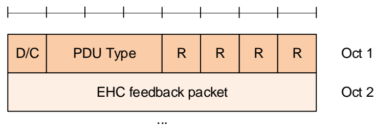
Figure 6.2.18.1: PDCCP Control PDU format for EHC feedback packet
