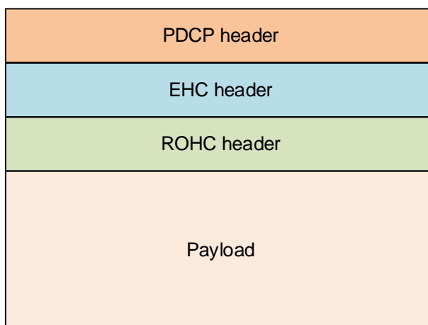
Figure 5.14.7.1: Location of ROHC header and EHC header in a PDCP Data PDU
