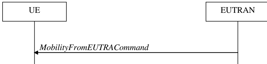
Figure 5.4.3.1-1: Mobility from E-UTRA, successful
