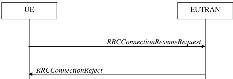
Figure 5.3.3.1-5: RRC connection resume or UP-EDT, network reject (suspended RRC connection or RRC_INACTIVE) or release (suspended RRC connection)
