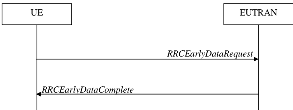
Figure 5.3.3.1-7: CP-EDT, successful
